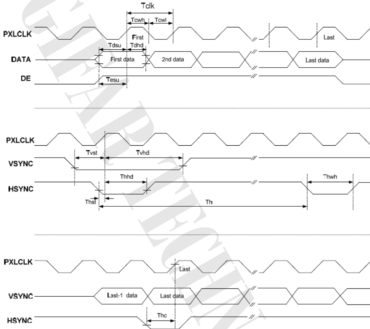
Fig.3-1 Clock and Data Input Timing Diagram
