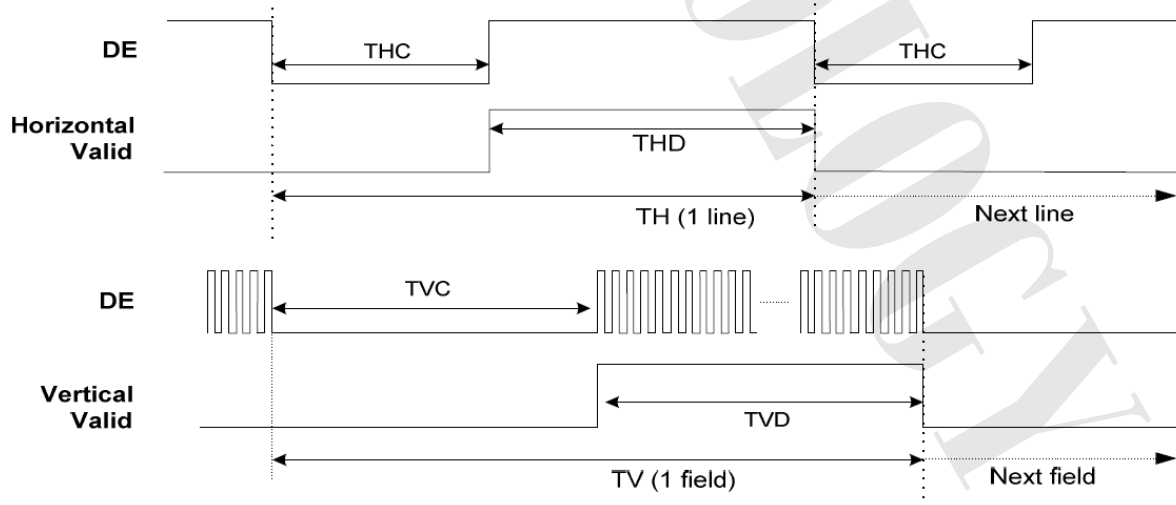
Fig.3-2 DE Mode Input Timing
