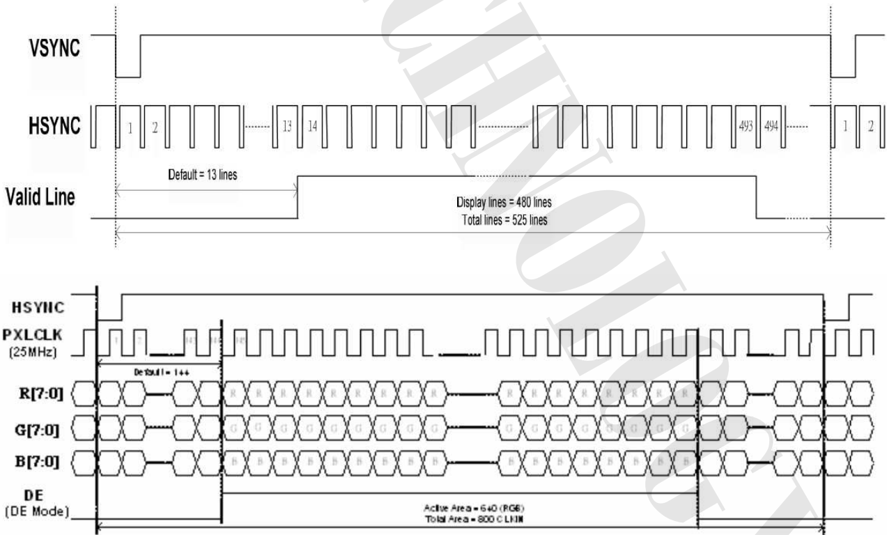
Fig. 3-4 24 bit RGB mode for 640 x (RGB) x 480
